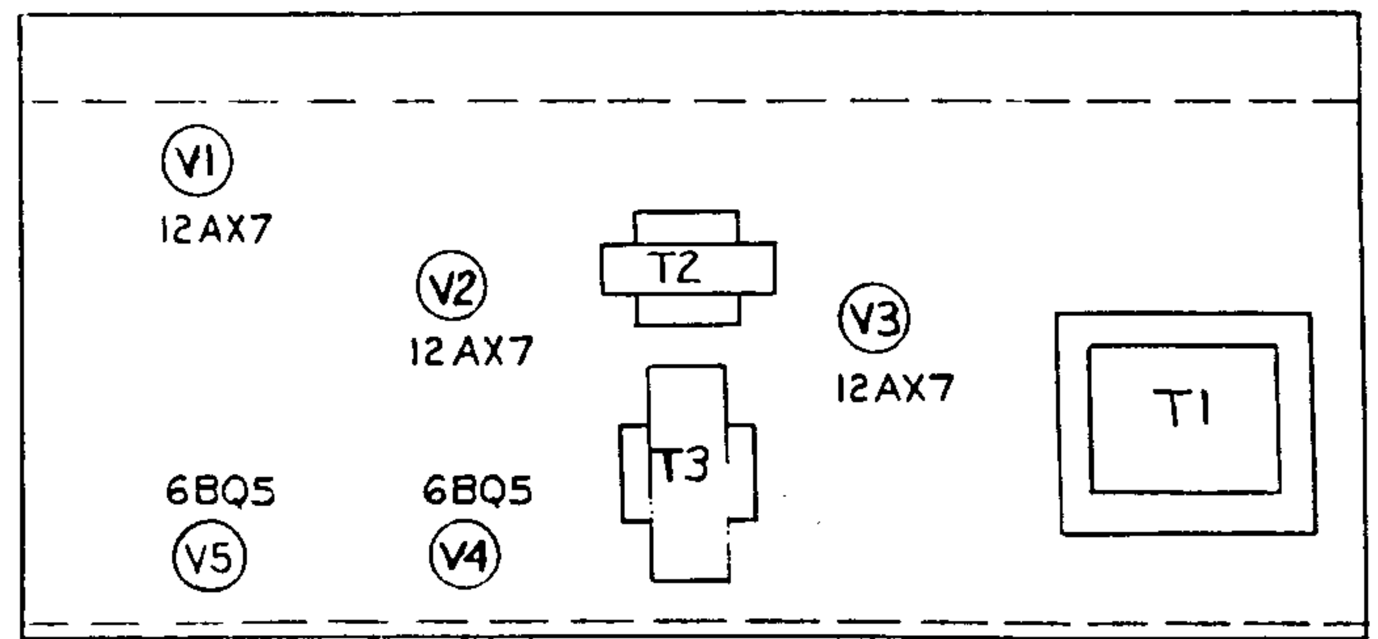
TUBE LOCATION CHART
