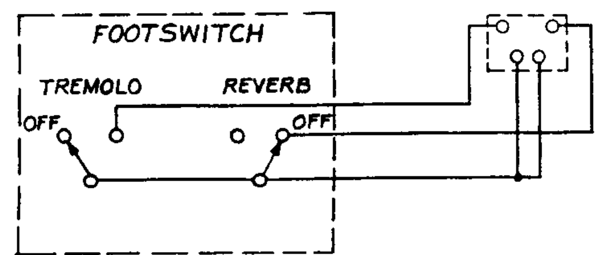
FOOTSWITCH & PLUG
