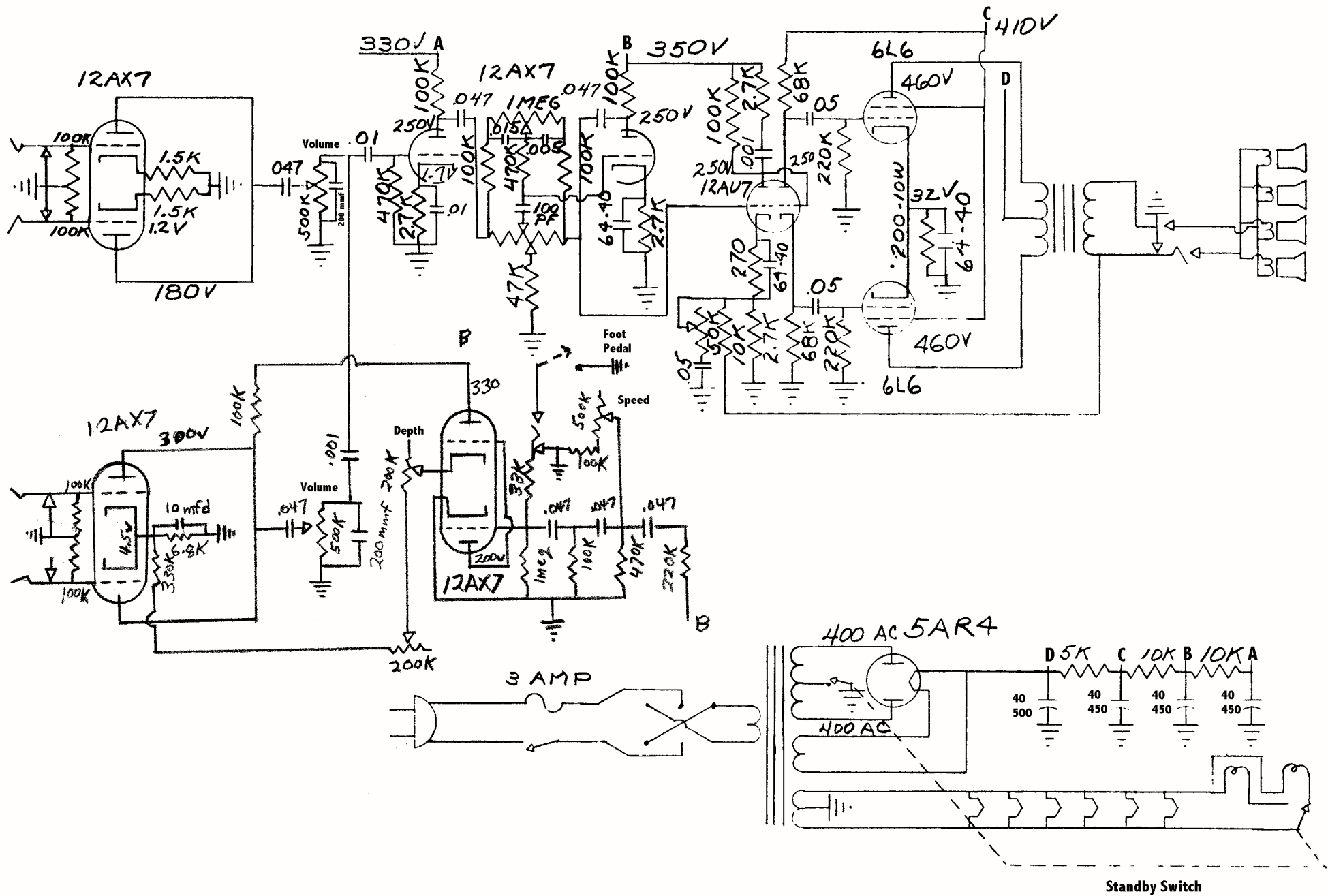
Model B16A, B16AD Amplifier
